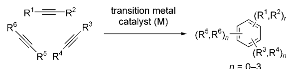
Scheme 1. Intermolecular crossed-cyclotrimerization of three different alkynes.
