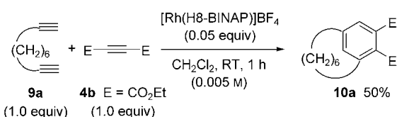
Scheme 6. Synthesis of a [6]metacyclophane by intermolecular crossed-cyclotrimerization of 1,9-decadiyne and DEAD.
