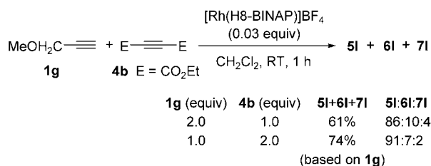
Scheme 10. Crossed-cyclotrimerization of 1g with excess 4b .
