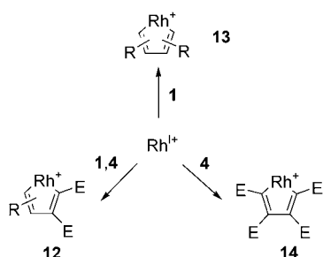
Scheme 7. Possible formation of rhodium metallacycles from 1 and 4 .
