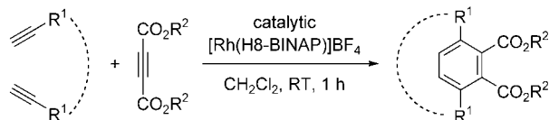
Scheme 2. Cationic rhodium(i)/H8-BINAP complex catalyzed chemo- and regioselective intermolecular crossed-cyclotrimerization of terminal alkynes and dialkyl acetylenedicarboxylates.
