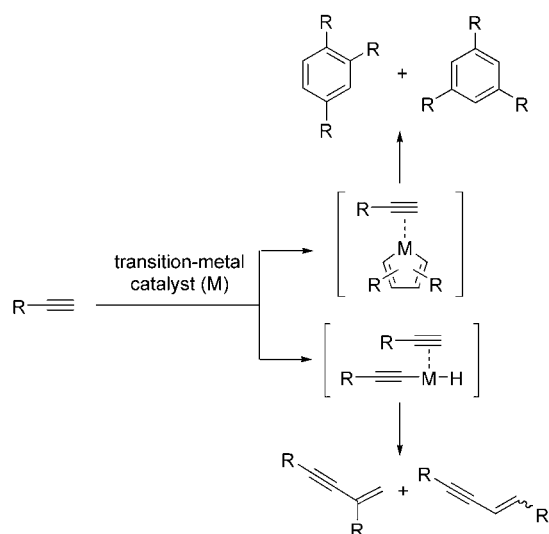
Scheme 3. Transition metal catalyzed dimerization and cyclotrimerization of terminal alkynes.
