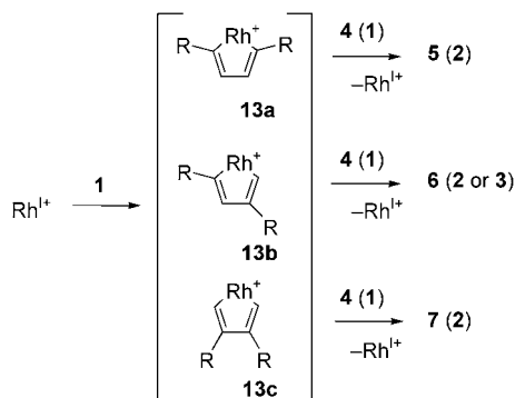
Scheme 9. Correlation of cyclotrimerization products with rhodium metallacycles 13a–c .
