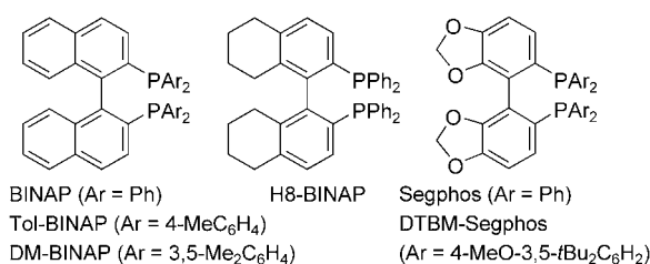
Scheme 5. Structures of modified BINAP ligands.
