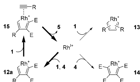
Scheme 11. Plausible mechanism for intermolecular crossed-cyclotrimerization of 1 and 4 catalyzed by the cationic rhodium(i)/H8-BINAP complex.
