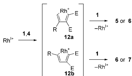
Scheme 8. Correlation of cyclotrimerization products with rhodium metallacycles 12a and 12b .
